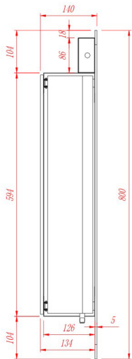
LEFT VIEW
