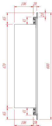
LEFT VIEW
